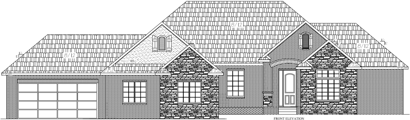
FRONT ELEVATION 1/4" = 1'
